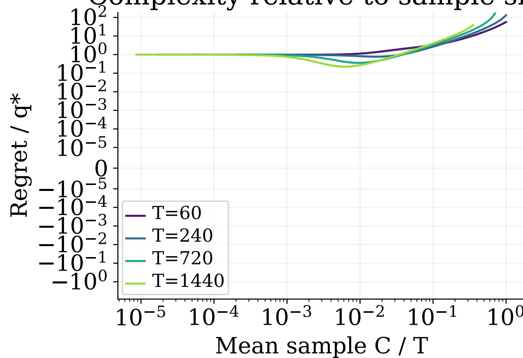
Complexity relative to sample size
