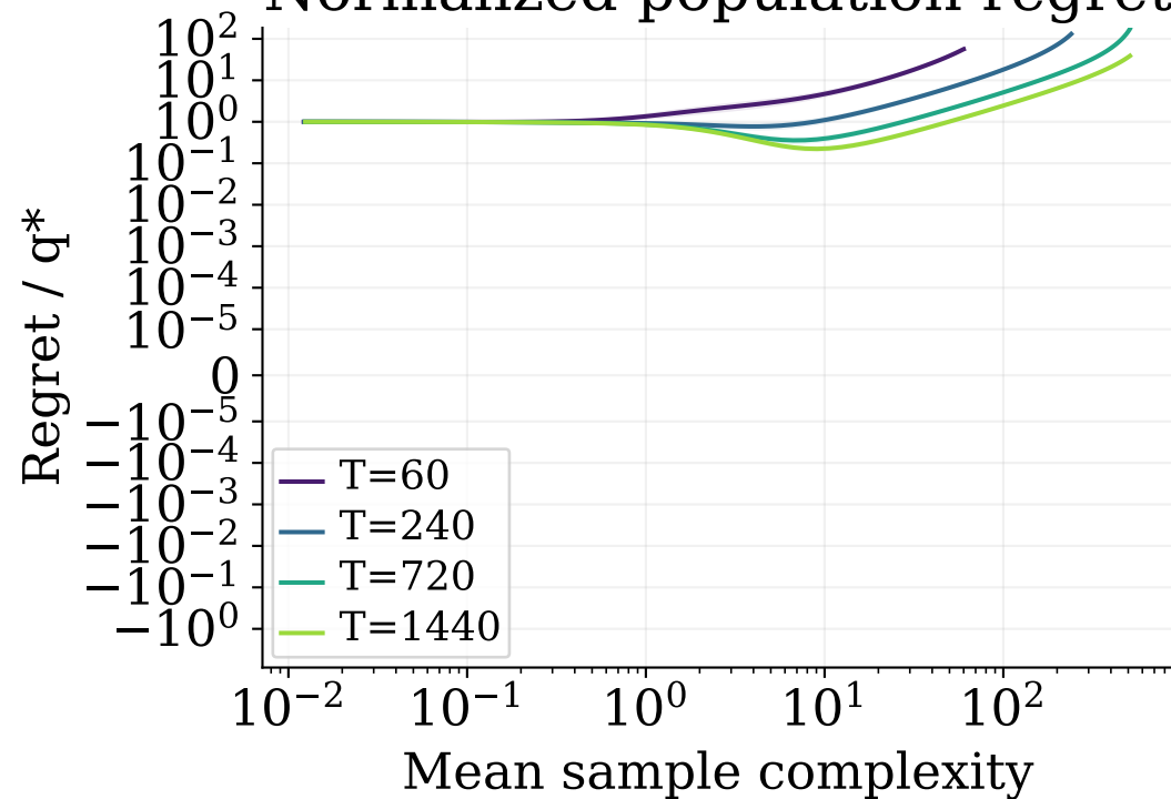
Normalized population regret
